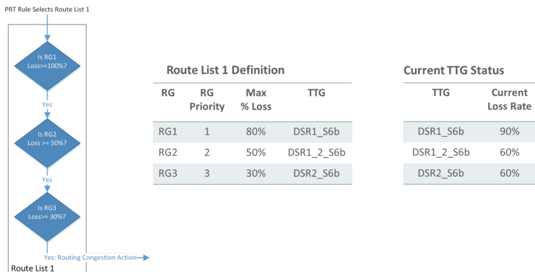
Figure 40 - Congestion-Aware Route List Logic Example 1b
