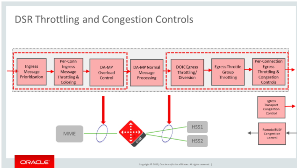
Figure 21 - Congestion Control
