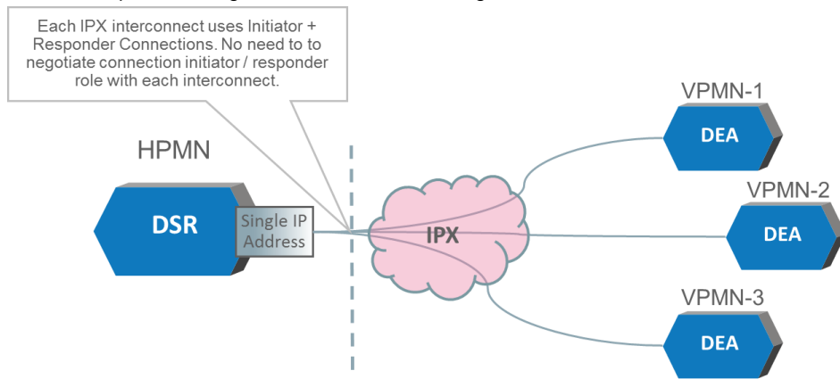
Figure 42 - IPFE Initiator or Responder Support
