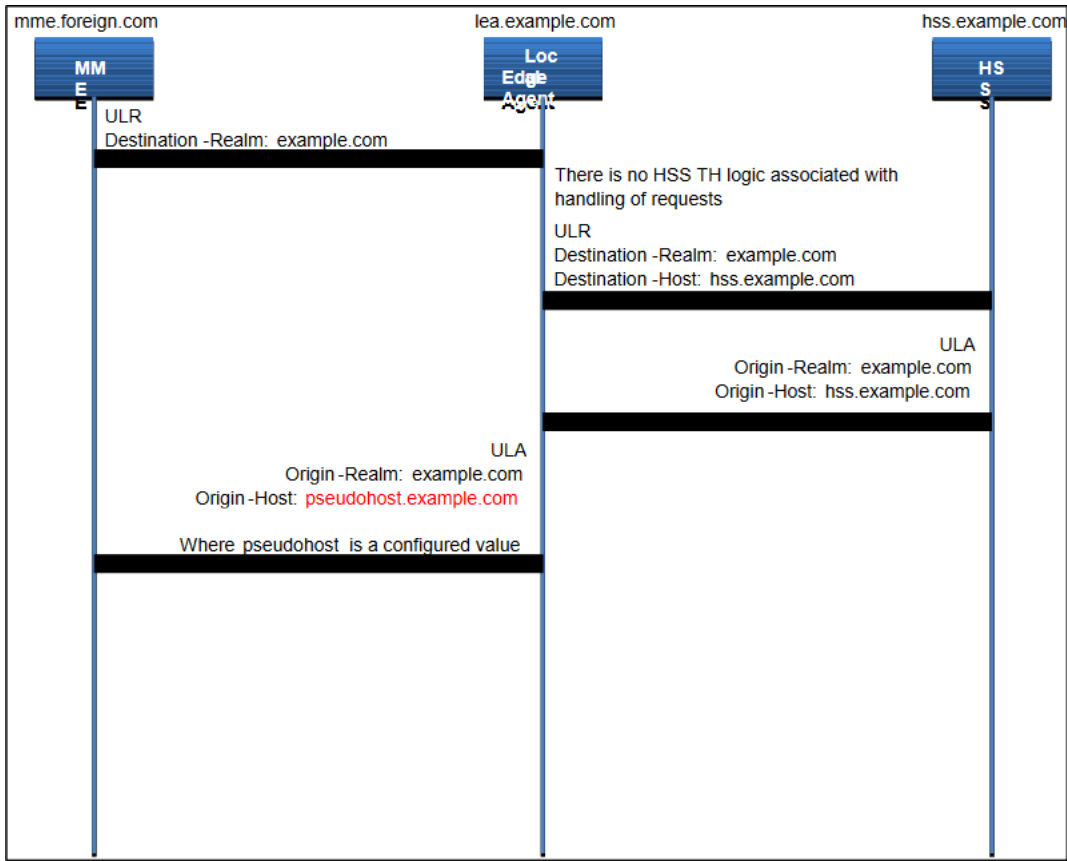
Figure 50 - S6a/S6d HSS Topology Hiding - ULR Message Flow
