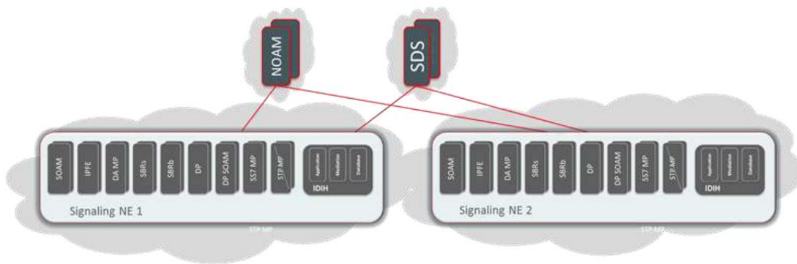
Figure 76 – DSR Architecture with STP VNF Message Processor
