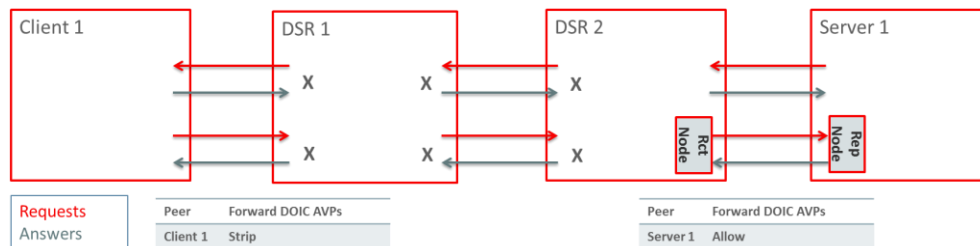
Figure 33 - DOIC Security Setting Example
