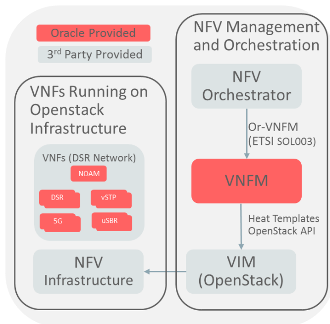
Figure 69 – DSR VNFM
