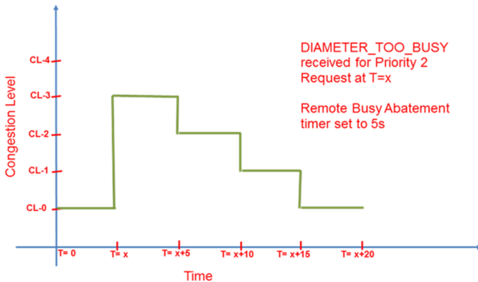
Figure 29 – Congestion level abatement over time for Remote Busy
