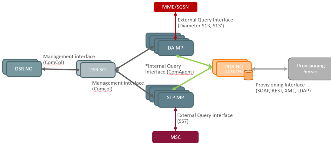
Figure 77 – EIR solution architecture.
